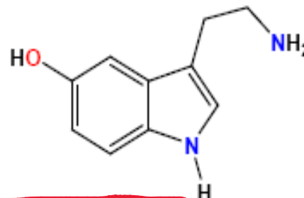
5-hydroxytryptamine (serotonin)
