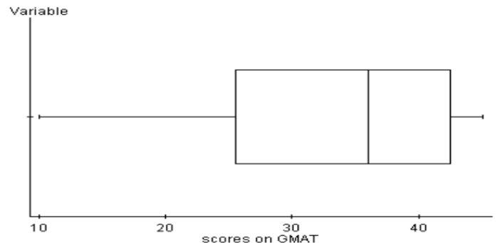
Boxplot
