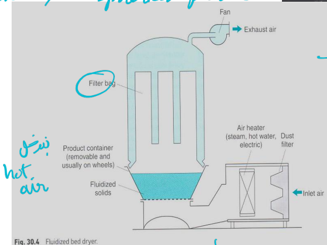
Fig. 30.4 Fluidized bed dryer.
