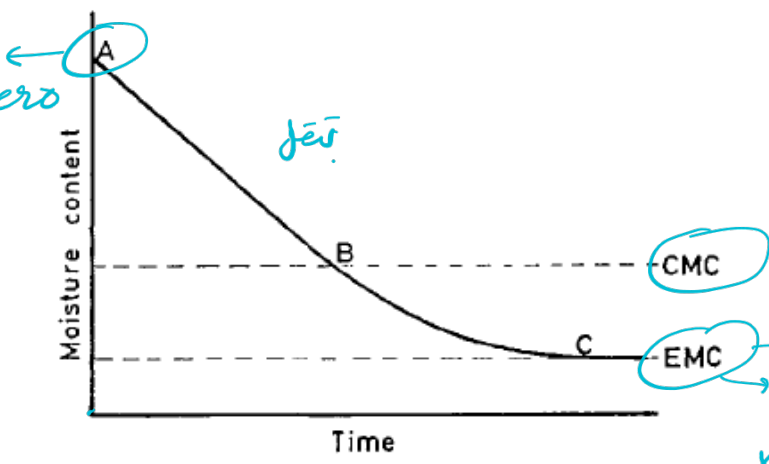
Fig. 26.5 Drying curve. CMC, critical moisture content, EMC, equilibrium moisture content.
